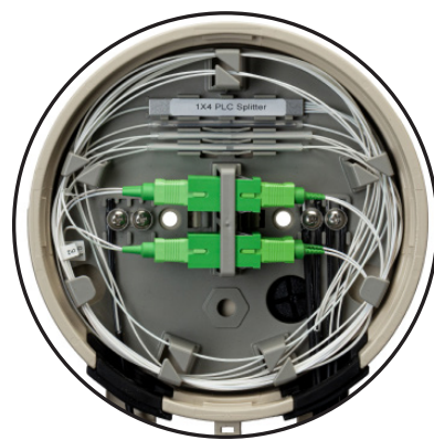
SC-APC Installation
