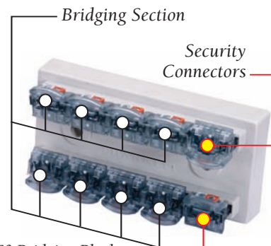
MRSB-10-F0 Bridging Block
